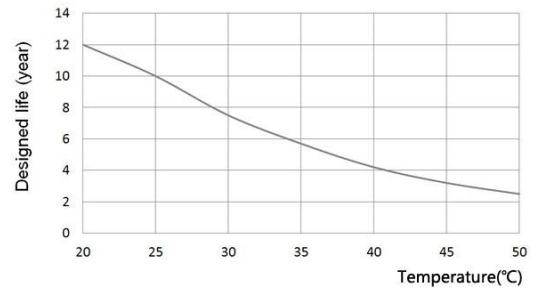
Design life Vs temperature
