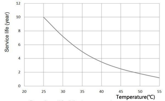
Service life Vs temperature
